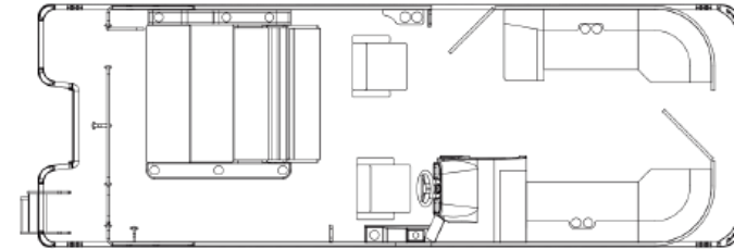
24' Legacy Swingback
