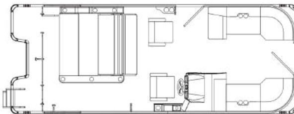
22' Legacy Swingback
